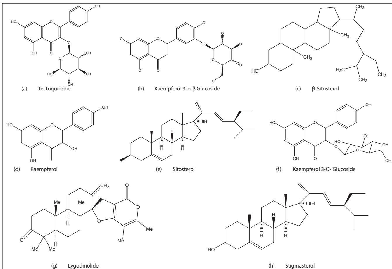
Figure 4 (a-h): Structures of the chemical compounds found in Lygodium flexuosum
